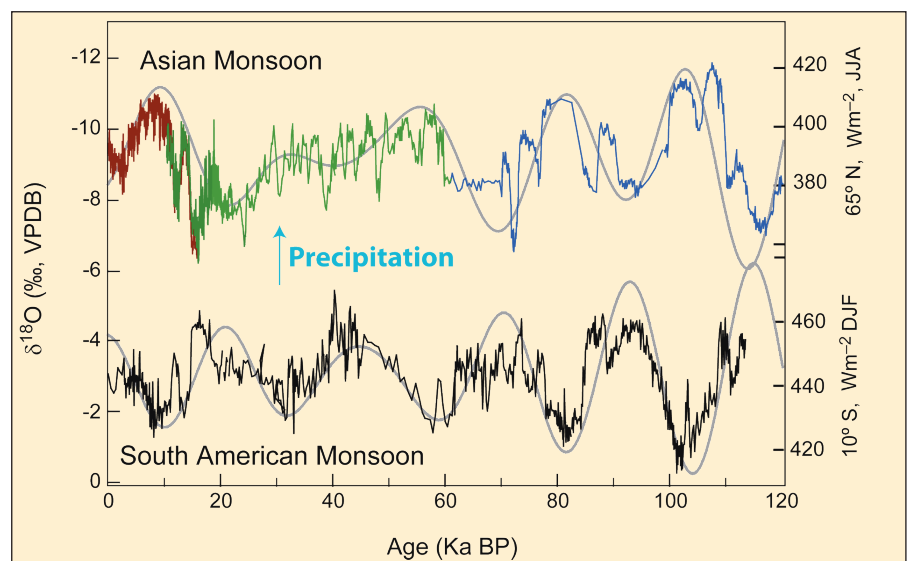
Figure 1: Interhemispheric comparison of changes in monsoon precipitation and summer insolation between eastern Asia and South America. Precipitation changes are reflected in \delta^{18}\text{O} records of speleothem calcite from Dongge cave (brown; Dykoski et al., 2005), Hulu cave (green; Wang et al., 2001), and Sanbao cave (blue; Wang et al., 2008) from eastern China, and from Botuverá cave in southern Brazil (black; Cruz et al., 2005). Insolation data are from (Berger, 1978). Figure courtesy of Hai Cheng.
